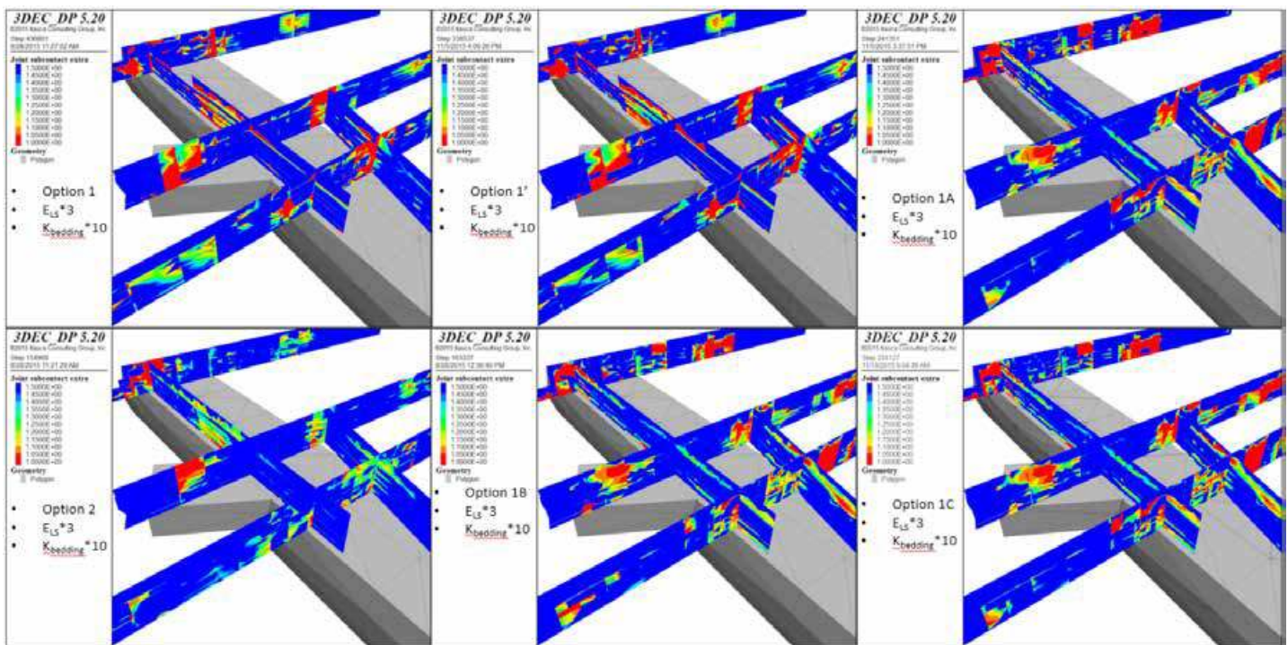
Figure 7. Predicted factor of safety against slip for selected vertical joints near the Transit Center connection after excavation and column loads: Option 1 model (upper left); Option 1' model (upper center); Option 1A model (upper right); Option 2 model (lower left); Option 1B model (lower center); and Option 1C model (lower right). (Red is FoS = 1.0 and blue is FoS \geq 1.5.) 1
