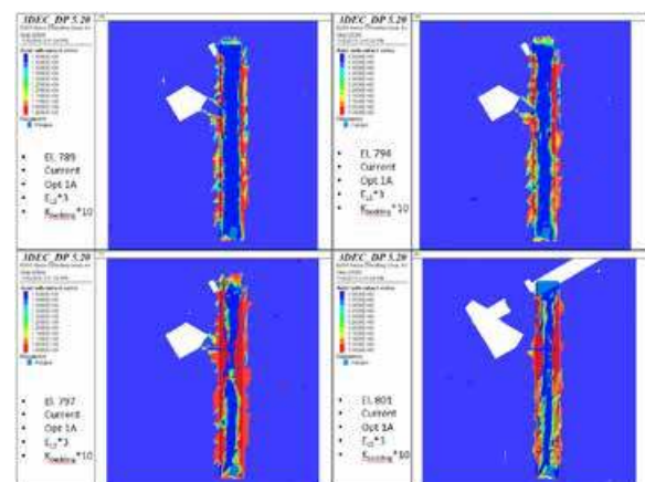
Figure 8. Predicted factor of safety against slip for the current station condition for the bedding planes at elevation 789 (upper left), 794 (upper right), 797 (lower left), and 801 (lower right).
