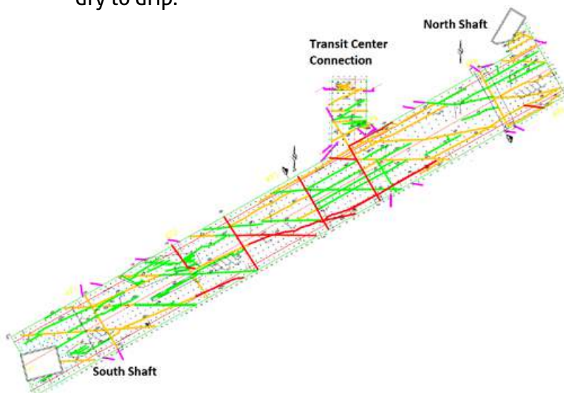
Figure 3. Platteville limestone joints mapped during construction.
