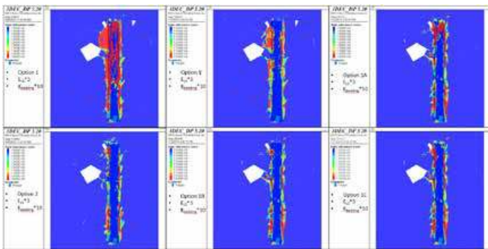
Figure 9. Predicted factor of safety against slip for the bedding plane at elevation 789: Option 1 model (upper left); Option 1' model (upper center); Option 1A model (upper right); Option 2 model (lower left); Option 1B model (lower center); and Option 1C model (lower right).
