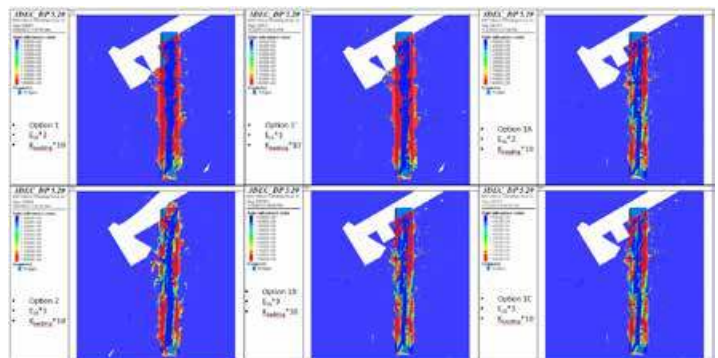
Figure 12. Predicted factor of safety against slip for the bedding plane at elevation 801: Option 1 model (upper left); Option 1' (upper center); Option 1A (upper right); Option 2 (lower left); Option 1B (lower center); and Option 1C (lower right).
