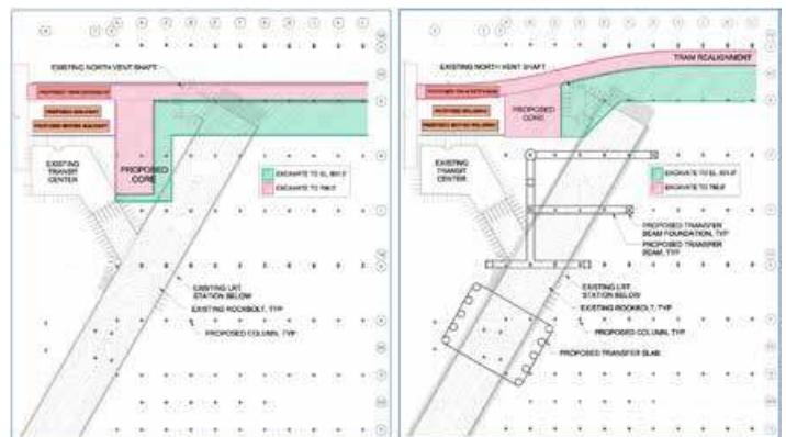
Figure 4. Layout of Option 1 (left) and Option 2 (right).
