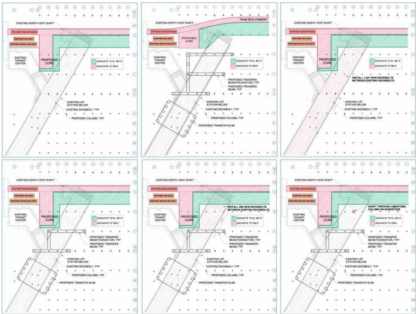
Figure 5. Layout of six options studied, top row left to right: Option 1, Option 2, Option 1'; bottom row left to right: Option 1A, Option 1B, Option 1C.
