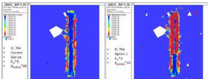
Figure 13. Comparison of factor of safety for the bedding plane at 794: current condition (left); Option 1 (right).
