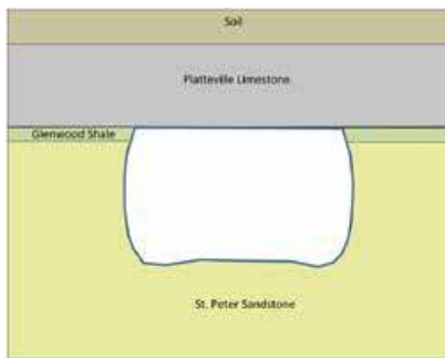
Figure 1. Geologic cross-section at the LRT station.
