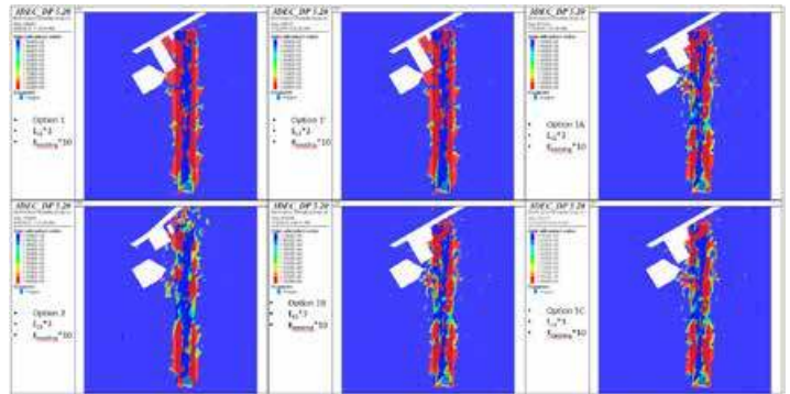
Figure 10. Predicted factor of safety against slip for bedding plane at elevation 794: Option 1 model (upper left); Option 1' (upper center); Option 1A (upper right); Option 2 (lower left); Option 1B (lower center); and Option 1C (lower right).
