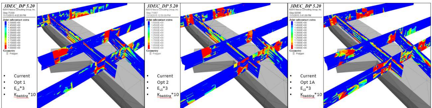
Figure 6. Predicted factor of safety against slip for selected vertical joints near the Transit Center connection for the current station state: Option 1 model (left); Option 2 model (center); and Option 1A model (right). (Red is FoS = 1.0 and blue is FoS \geq 1.5 .)
