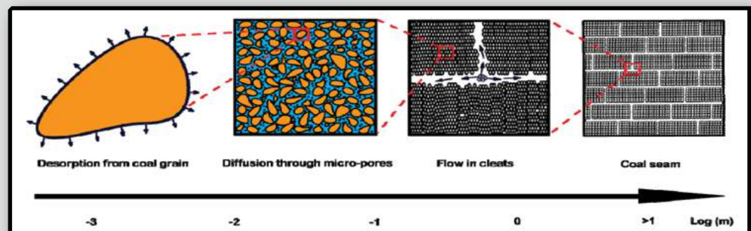
Figure 1: Migration process of gas in dual porosity coal seams
