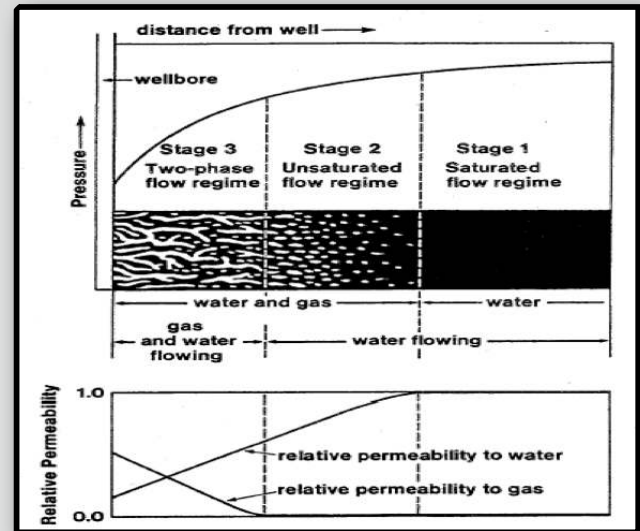
Figure 2: Three stages of coalbed gas production.
