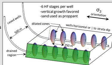
Figure 1: Multiple HF stages for shale gas stimulation.
