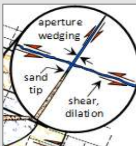
Figure 2: Fracture opening (dilation) created by wedging and shear displacement.
