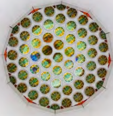
Figure 2: Inside the Large Underground Xenon (LUX) dark matter detector, with photomultiplier tubes (PMTs) at the top and bottom of the detector
